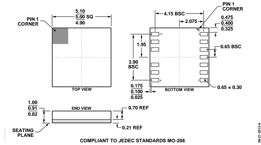
COMPLIANT TO JEDEC STANDARDS MO-208 Figure 23. 13-Terminal Land Grid Array [LGA] (CC-13-1) Dimensions shown in millimeters
